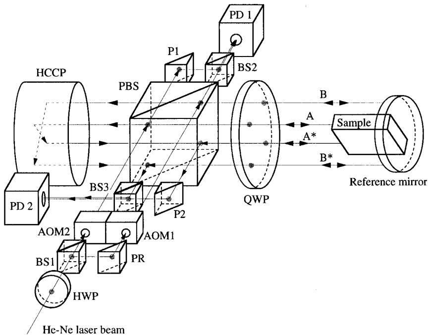
Fig. 3. Schematic diagram of the double-path optical heterodyne interferometer consisting of the following optical elements: acousto-optical modulators AOM1 and AOM2, beam splitters BS1, BS2, and BS3, half-wave plate HWP, hollow cube corner prism HCCCP, photodetectors PD1 and PD2, plane reflector PR, polarized beam splitter PBS, prisms P1 and P2, quarter-wave plate QWP.
